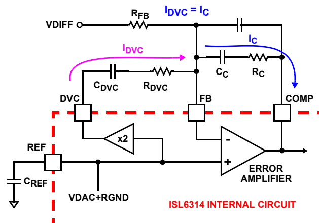
FIGURE 8. VID-ON-THE-FLY COMPENSATION NETWORK
