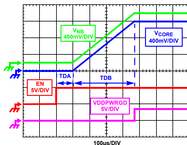
FIGURE 13. SOFT-START WAVEFORMS
