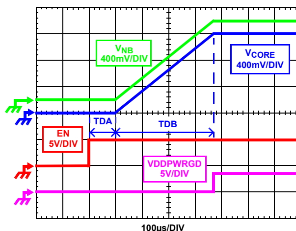
FIGURE 11. SOFT-START WAVEFORMS
