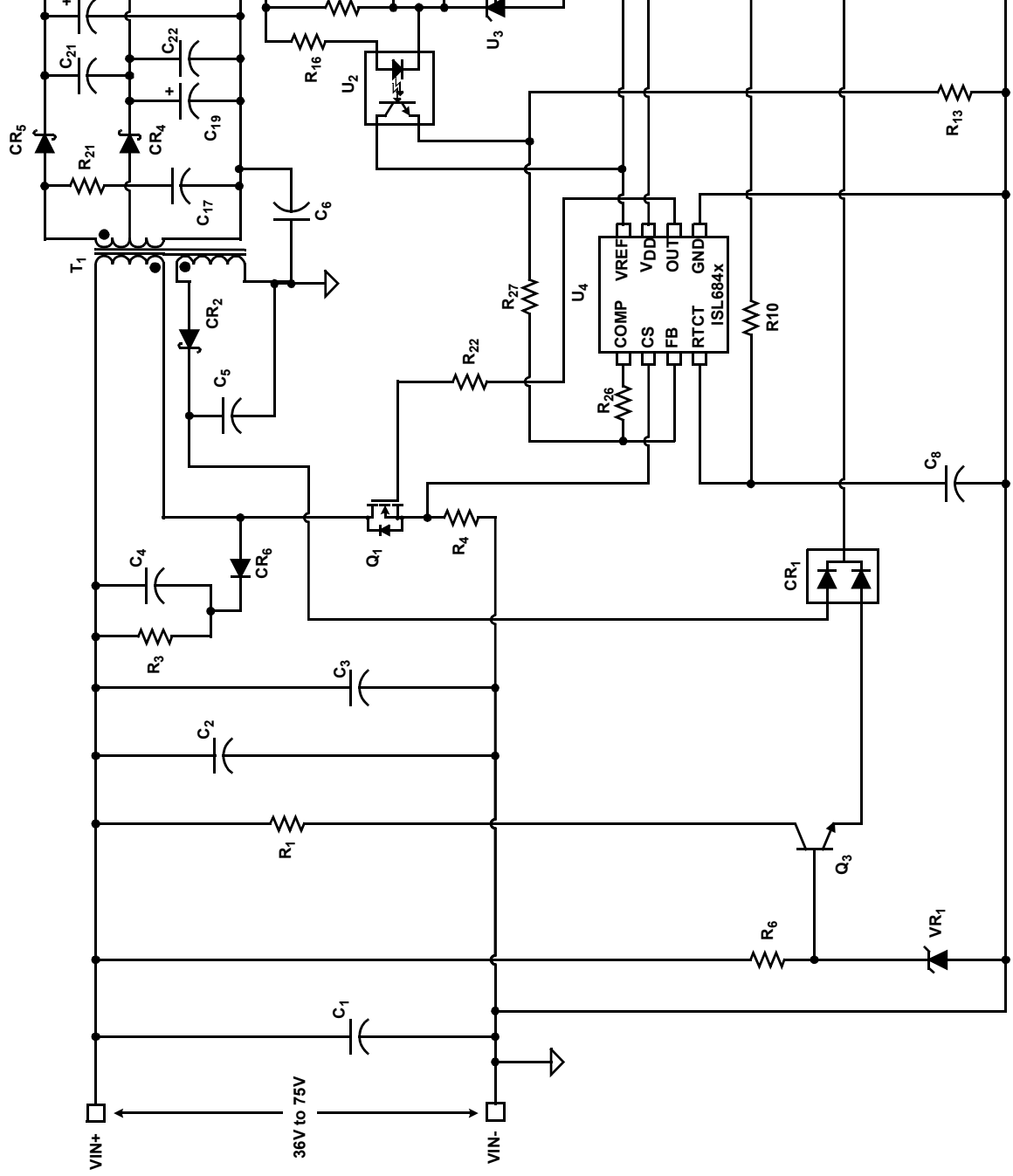
Figure 1. 48V Input Dual Output Flyback
