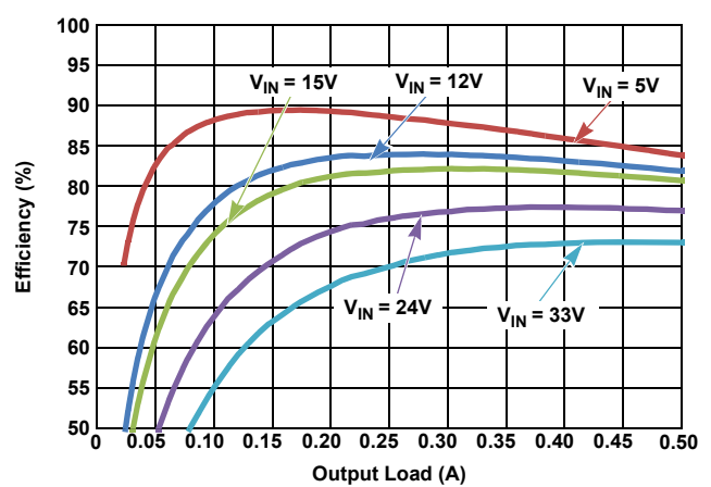
Figure 11. Efficiency vs Load, PWM, V_{OUT} = 1.8V
