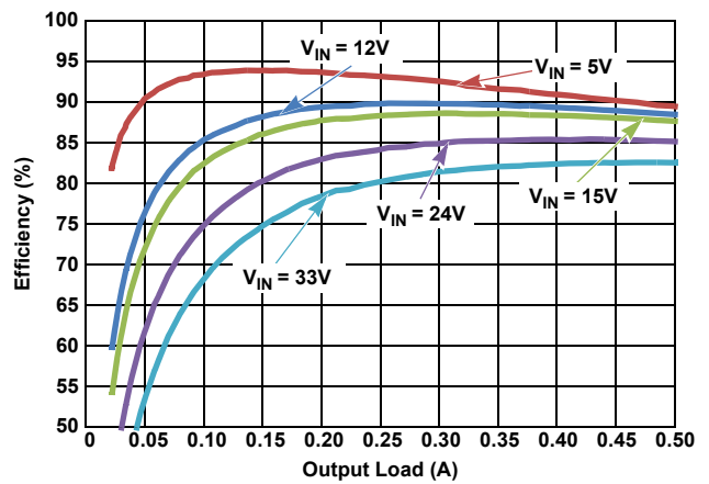
Figure 21. Efficiency vs Load, PMW, V_{OUT} = 3.3V
