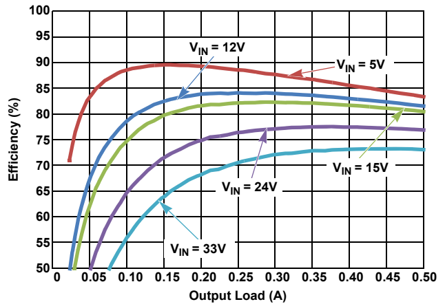
Figure 23. Efficiency vs Load, PMW, V_{OUT} = 1.8V
