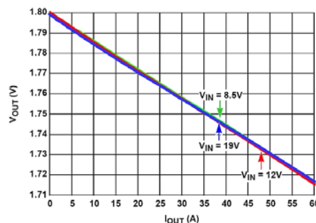
FIGURE 1. LOAD LINE REGULATION
