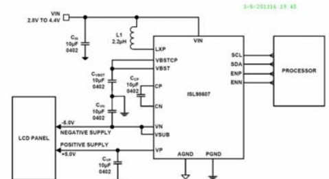
FIGURE 1. TYPICAL APPLICATION CIRCUIT: TFT-LCD SMART PHONE DISPLAY
