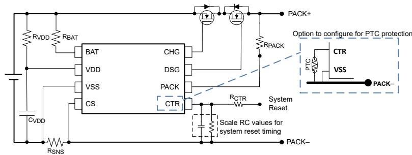
Simplified Schematic
