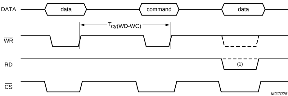
Fig 22. Write data + write command cycle timing.
