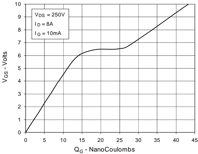
Fig. 9. Gate Charge
