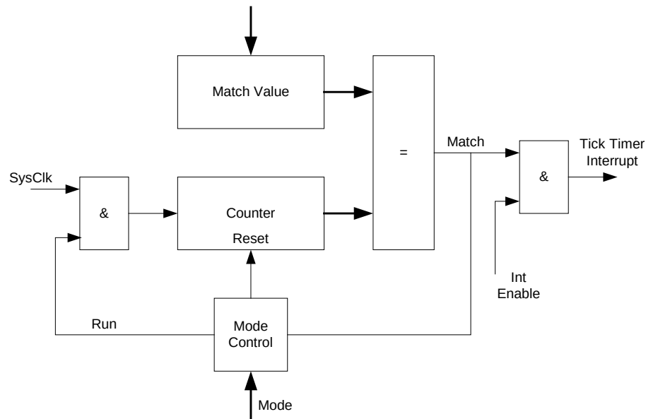
Figure 31 Tick Timer
