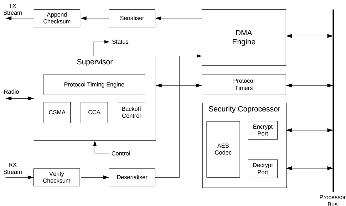
Figure 19: Baseband Processor
