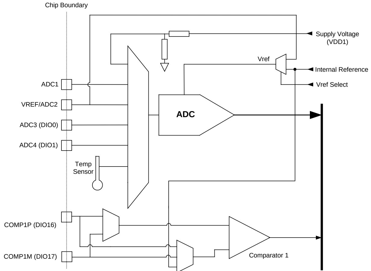
Figure 37: Analogue Peripherals
