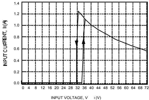
Figure 1. Typical JW050F Input Characteristics at Room Temperature
