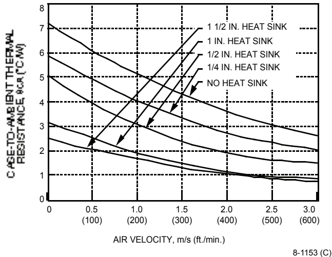
Figure 32. Case-to-Ambient Thermal Resistance Curves; Either Orientation
