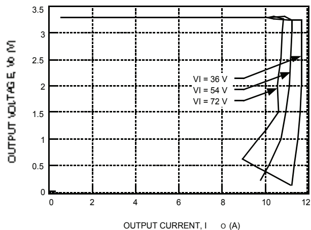
Figure 5. Typical JW050F Output Characteristics at Room Temperature
