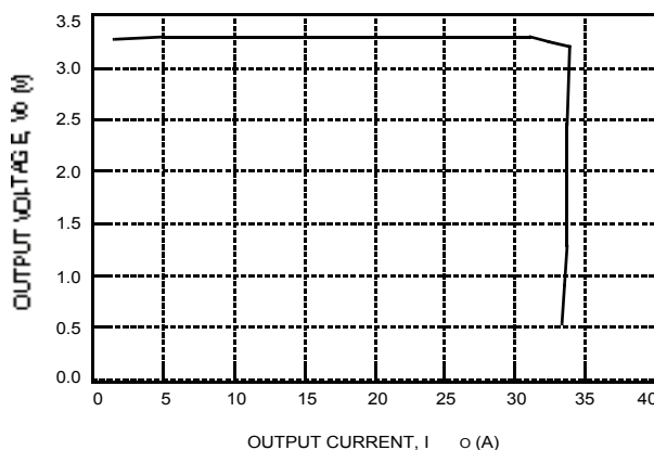
Figure 8. Typical JW150F Output Characteristics at Room Temperature
