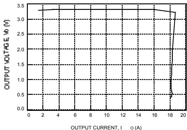
Figure 6. Typical JW075F Output Characteristics at Room Temperature
