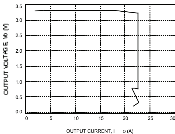
Figure 7. Typical JW100F Output Characteristics at Room Temperature
