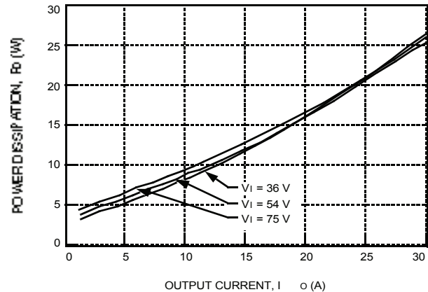
Figure 30. JW150F Power Dissipation vs. Output Current
