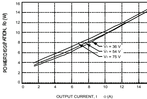
Figure 28. JW075F Power Dissipation vs. Output Current
