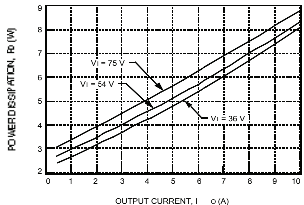
Figure 27. JW050F Power Dissipation vs. Output Current
