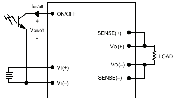
Figure 20. Remote On/Off Implementation
