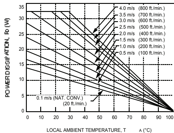
Figure 31. Forced Convection Power Derating with No Heat Sink; Either Orientation
