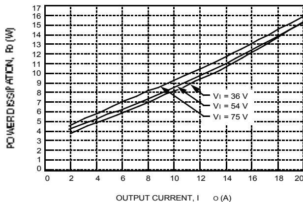
Figure 29. JW100F Power Dissipation vs. Output Current
