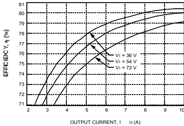
Figure 9. Typical JW050F Converter Efficiency vs. Output Current at Room Temperature
