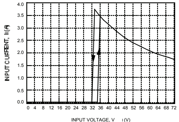
Figure 4. Typical JW150F Input Characteristics at Room Temperature
