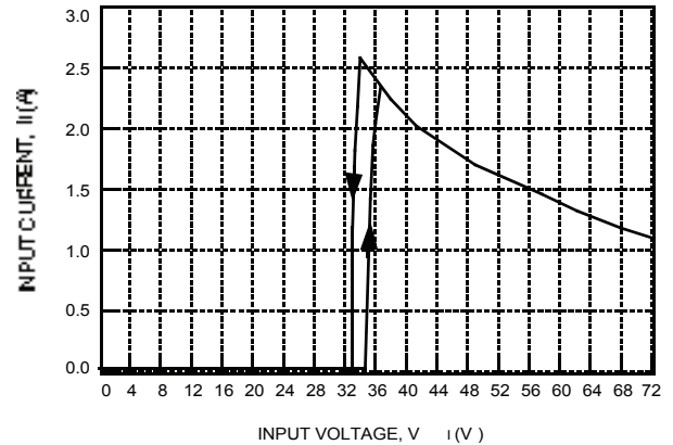
Figure 3. Typical JW100F Input Characteristics at Room Temperature
