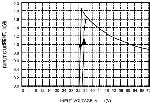
Figure 2. Typical JW075F Input Characteristics at Room Temperature
