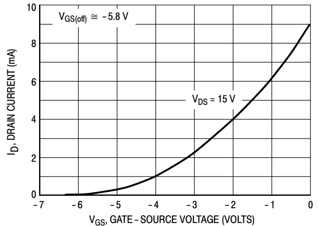
Figure 7. Common Source Transfer Characteristics
