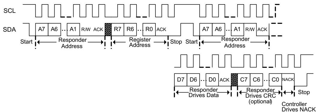
Figure 7-10. I²C Read Without Repeated Start
