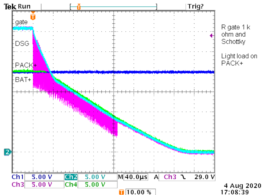
Figure 8-6. Moderate Speed DSG FET Turn-Off, Using a 1-k \Omega Series Gate Resistor, and a Light Load on PACK+
