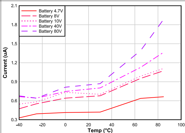
Figure 6-23. BAT Current in SHUTDOWN Mode vs. Temperature
