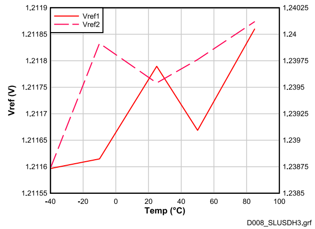
Figure 6-5. Internal Voltage References vs. Temperature (VREF1 and VREF2)
