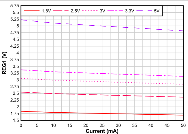
Figure 6-13. REG1 Voltage vs. Load at 25°C
