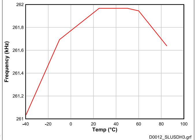
LFO measured in FULL SPEED mode (262 kHz) Figure 6-7. Low Frequency Oscillator (LFO) Accuracy vs. Temperature
