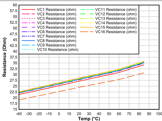
Figure 6-11. Cell Balancing Resistance vs. Temperature
