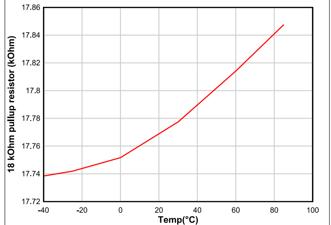
Figure 6-15. Thermistor Pullup Resistance vs. Temperature (18-kΩ Setting)
