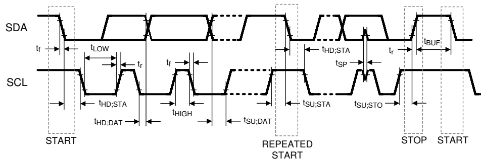
Figure 6-1. I²C Communications Interface Timing
