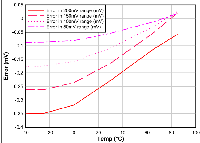
Figure 6-4. Current Measurement Error vs. Temperature
