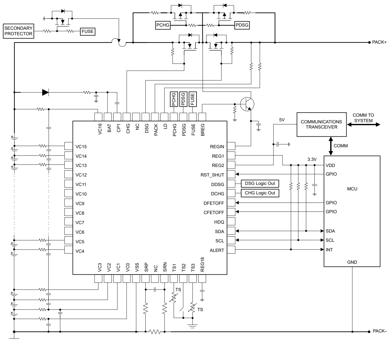
Figure 8-1. BQ76972 16-Series Cell Typical Implementation (Simplified Schematic)
