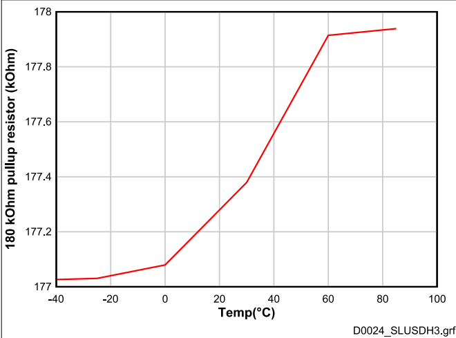
Figure 6-16. Thermistor Pullup Resistance vs. Temperature (180-kΩ Setting)
