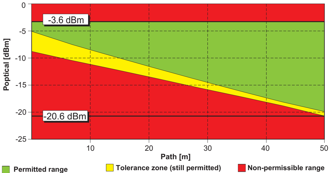
Limit Values for Polymer Fibers in Drag Chain Applications of Different Lengths (70 m System)
