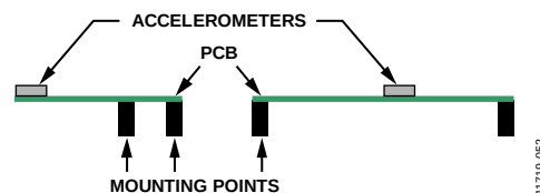
Figure 49. Incorrectly Placed Accelerometers
