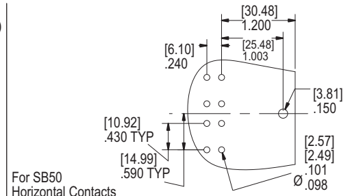
PCB Hole Layout for SB50
