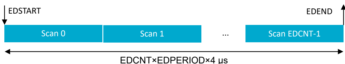
Figure 126: Energy detection measurement example with multiple iterations
