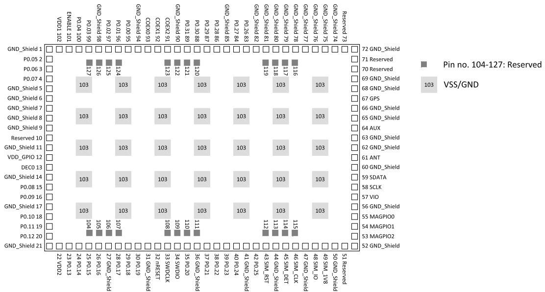
Figure 122: LGA pin assignments, top view
