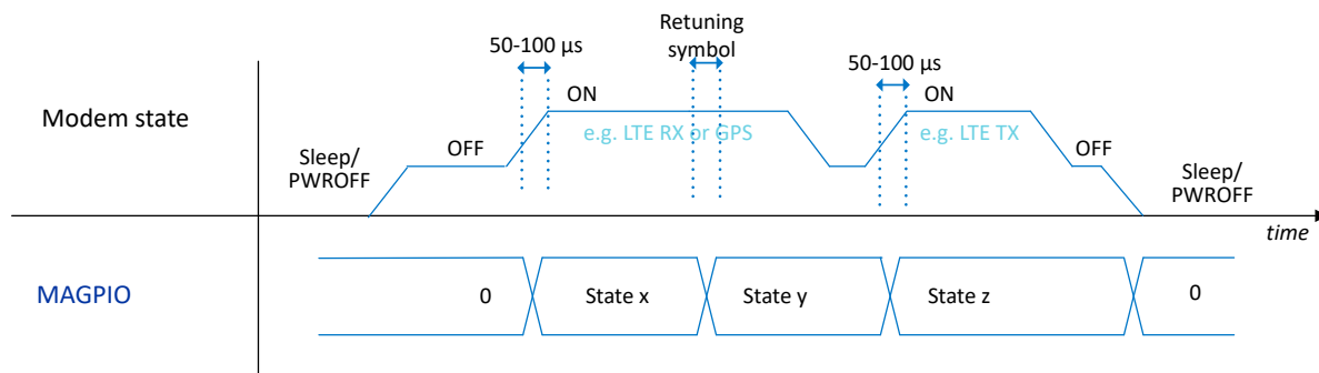
Figure 117: MAGPIO interface timing
