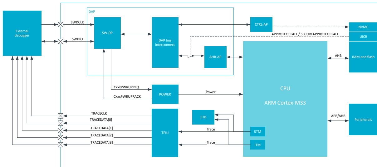
Figure 118: Debug and trace overview
