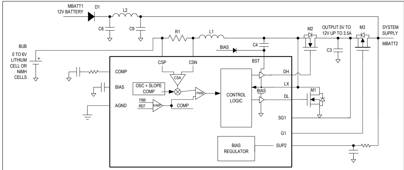
Figure 3. Boost Block Diagram
