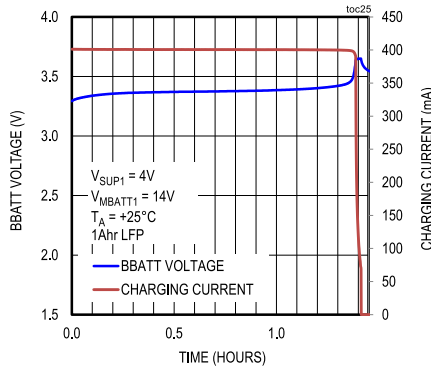
CHARGING PROFILE
