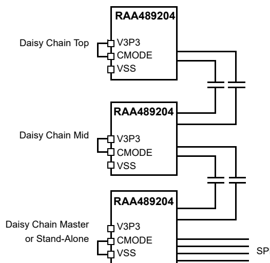
Figure 47. Communications Configuration
