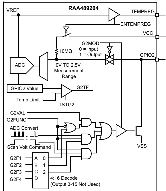
Figure 46. GPIO2 Block Diagram
