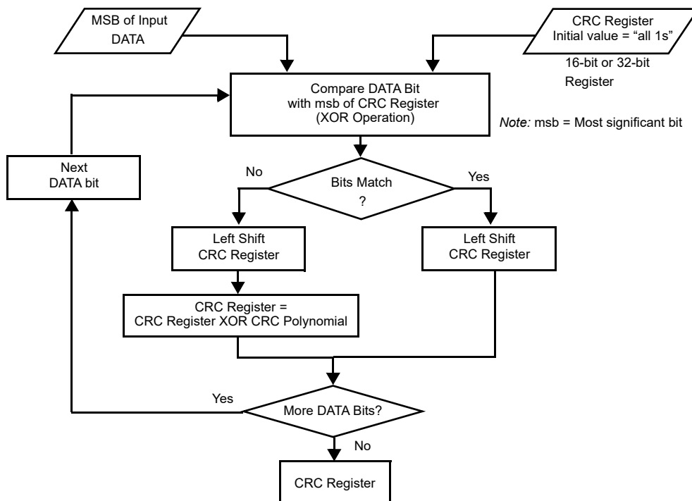
Figure 58. CRC Calculation
