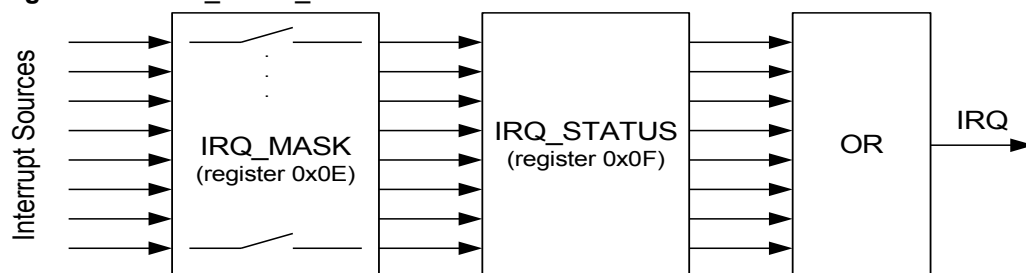
Figure 6-21. IRQ_MASK_MODE = 0.
