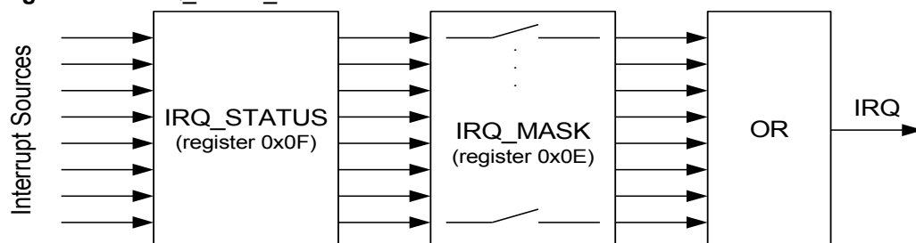
Figure 6-22. IRQ_MASK_MODE = 1.
