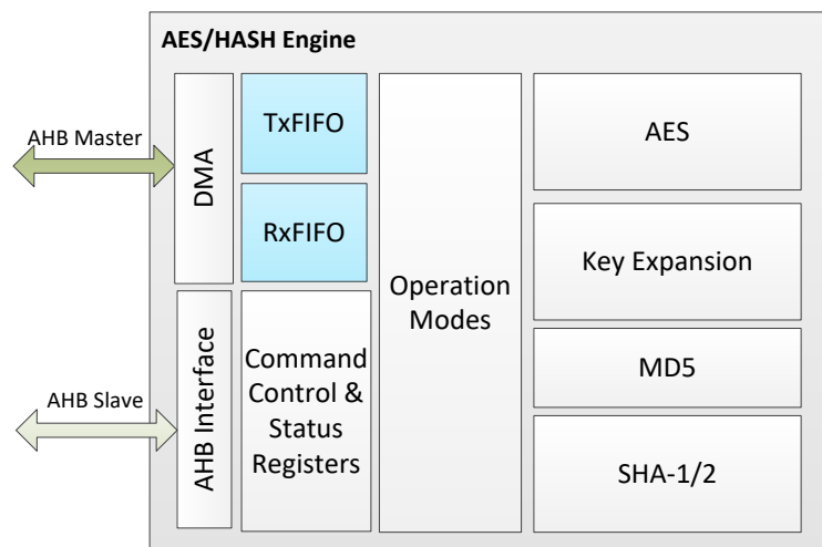
Figure 57. AES/HASH architecture
