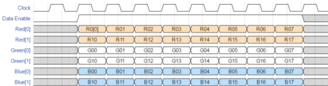
Figure 54. HSYNC/VSynch color bits waveform
