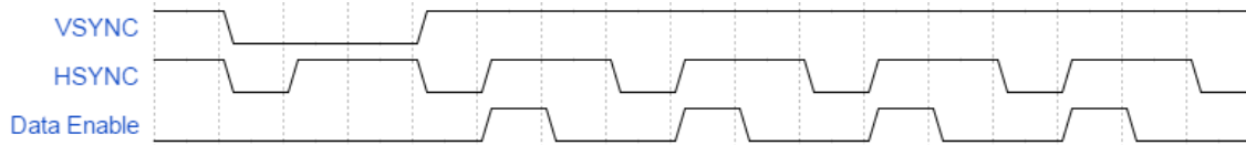
Figure 53: HSYNC/VSynch Typical Waveform
