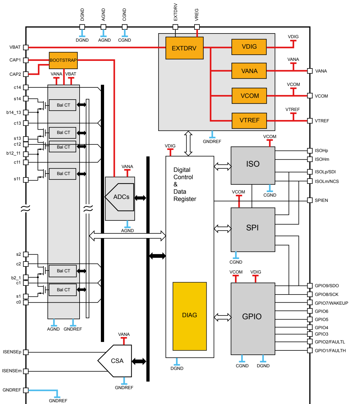
Figure 2. Block diagram
