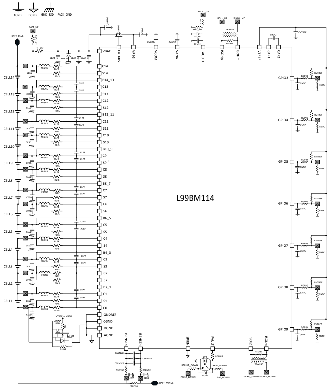
Figure 1. Typical application
