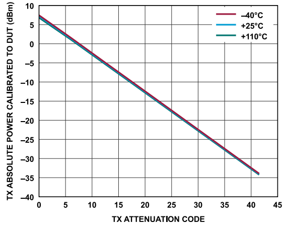
Figure 201. Transmitter Absolute Power Calibrate to DUT vs. Transmitter Attenuation Code, Baseband Frequency = 18 MHz, Backoff = 0.2 dBFS
