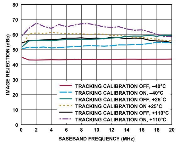
Figure 203. Transmitter Image Rejection vs. Baseband Frequency, Tracking Calibration On vs. Tracking Calibration Off, Transmitter Attenuation Code = 0
