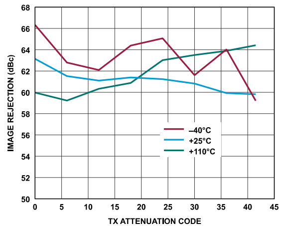
Figure 233. Transmitter Image Rejection vs. Transmitter Attenuation Code, Baseband Frequency = 2.1 kHz, Backoff = 0.2 dBFS
