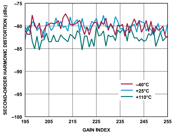
Figure 190. Receiver Second-Order Harmonic Distortion vs. Gain Index, Baseband Frequency = 5.6 MHz, ADC = Low Power
