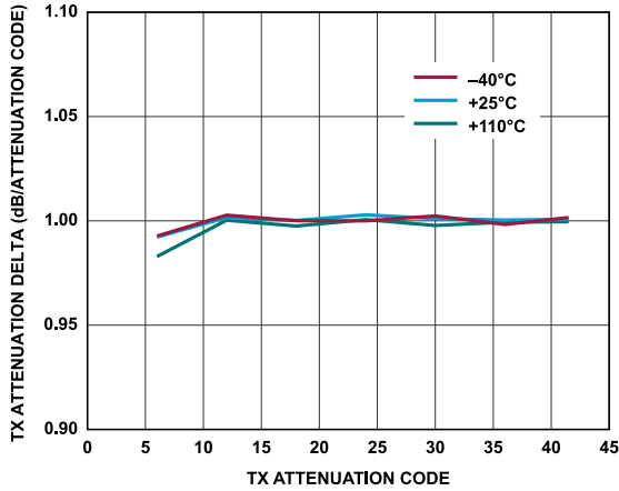
Figure 255. Transmitter Attenuation Delta vs. Transmitter Attenuation Code, Baseband Frequency = 2.1 kHz, Backoff = 0.2 dBFS
