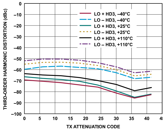
Figure 303. Transmitter Third-Order Harmonic Distortion vs. Transmitter Attenuation Code, Baseband Frequency = 2.1 kHz, Backoff = 0.2 dBFS
