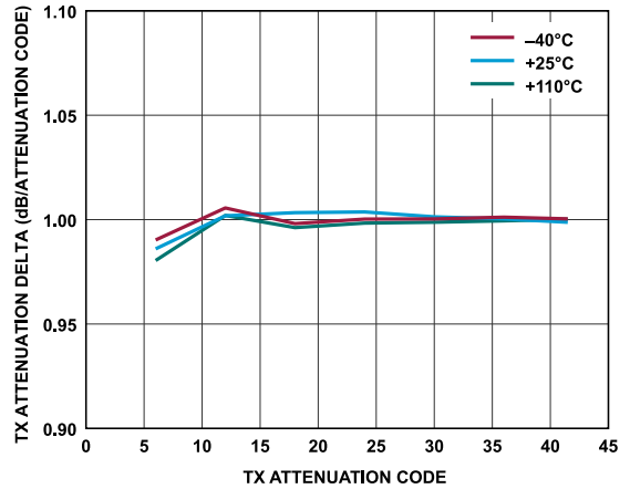
Figure 130. Transmitter Attenuation Delta vs. Transmitter Attenuation Code, Baseband Frequency = 18 MHz, Backoff = 0.2 dBFS
