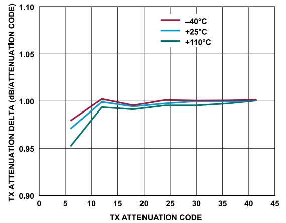
Figure 202. Transmitter Attenuation Delta vs. Transmitter Attenuation Code, Baseband Frequency = 18 MHz, Backoff = 0.2 dBFS
