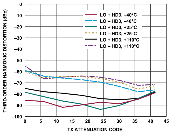
Figure 101. Transmitter Third-Order Harmonic Distortion vs. Transmitter Attenuation Code, Baseband Frequency = 18 MHz, Backoff = 0.2 dBFS
