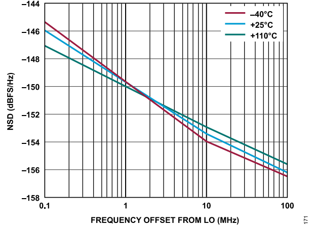
Figure 75. Transmitter NSD vs. Frequency Offset from LO, Baseband Frequency = 5.6 MHz, Transmitter Channel = Channel 1
