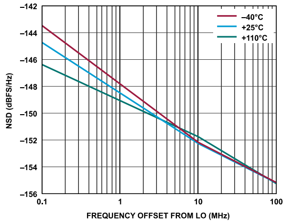
Figure 353. Transmitter NSD vs. Frequency Offset from LO, Baseband Frequency = 2.1 kHz, Transmitter Channel = Channel 1
