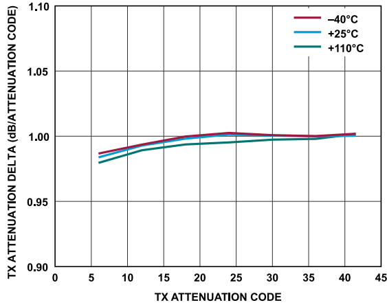
Figure 301. Transmitter Attenuation Delta vs. Transmitter Attenuation Code, Baseband Frequency = 2.1 kHz, Backoff = 0.2 dBFS
