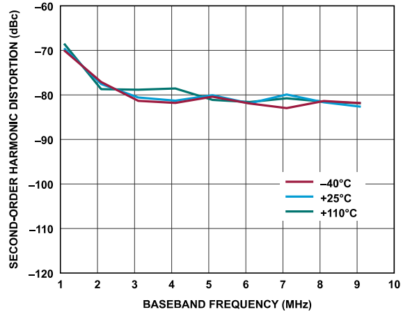
Figure 189. Receiver Second-Order Harmonic Distortion vs. Baseband Frequency, Gain Index = 255, ADC = High Performance
