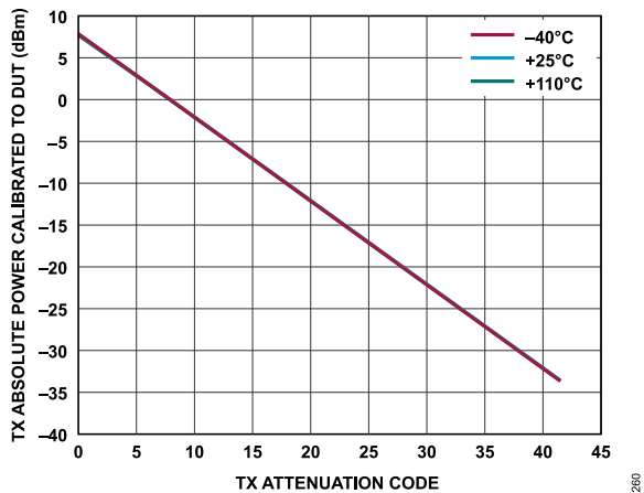
Figure 168. Transmitter Absolute Power Calibrated to DUT vs. Transmitter Attenuation Code, Baseband Frequency = 18 MHz, Backoff = 0.2 dBFS
