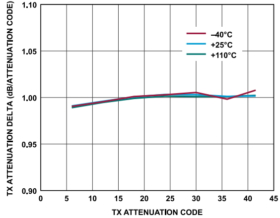
Figure 232. Transmitter Attenuation Delta vs. Transmitter Attenuation Code, Baseband Frequency = 2.1 kHz, Backoff = 0.2 dBFS
