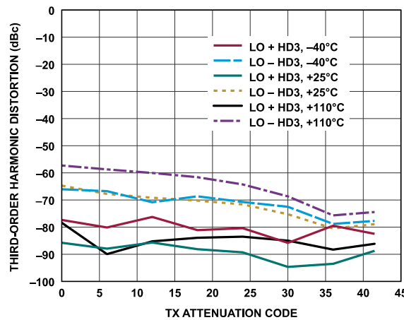
Figure 234. Transmitter Third-Order Harmonic Distortion vs. Transmitter Attenuation Code, Baseband Frequency = 2.1 kHz, Backoff = 0.2 dBFS, Initialization Calibration Only
