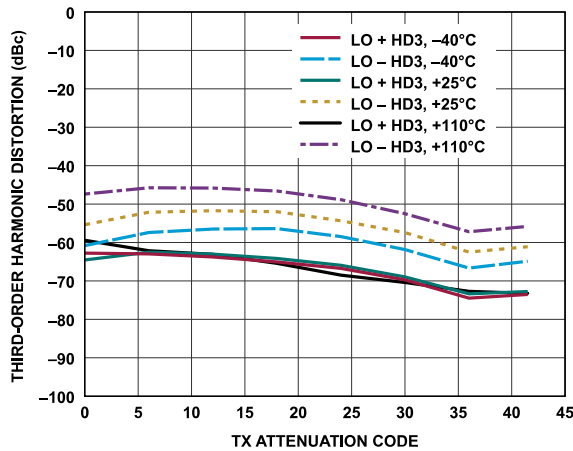
Figure 350. Transmitter Third-Order Harmonic Distortion vs. Transmitter Attenuation Code, Baseband Frequency = 2.1 kHz, Backoff = 0.2 dBFS
