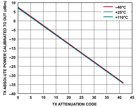
Figure 129. Transmitter Absolute Power Calibrated to DUT vs. Transmitter Attenuation Code, Baseband Frequency = 18 MHz, Backoff = 0.2 dBFS
