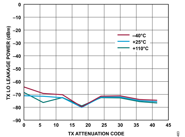
Figure 329. Transmitter LO Leakage Power vs. Transmitter Attenuation Code, Baseband Frequency = 2.1 kHz, Backoff = 6 dBFS, Initialization Calibration Only
