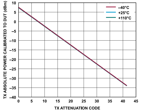
Figure 96. Transmitter Absolute Power Calibrated to DUT vs. Transmitter Attenuation Code, Baseband Frequency = 18 MHz, Backoff = 0.2 dBFS
