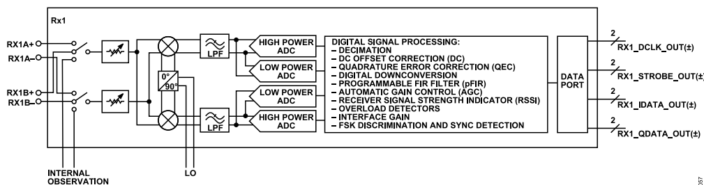
Figure 361. Receiver Architecture
