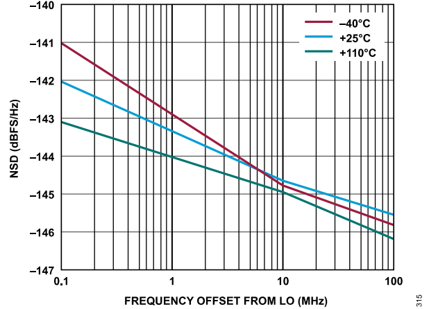
Figure 213. Transmitter NSD vs. Frequency Offset from LO, Baseband Frequency = 5.6 MHz, Transmitter Channel = Channel 1
