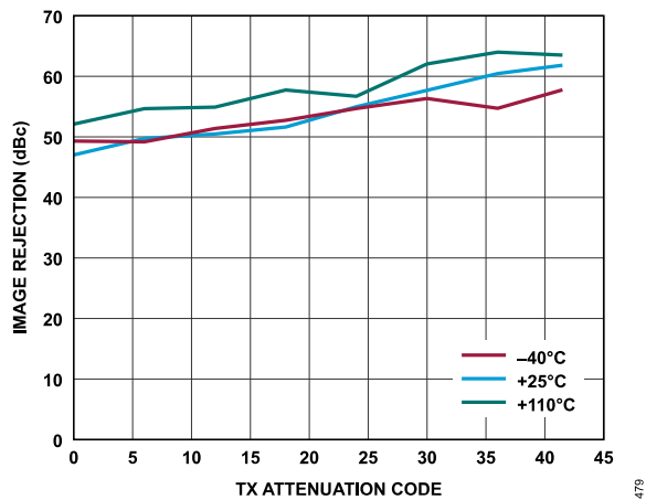
Figure 326. Transmitter Image Rejection vs. Transmitter Attenuation Code, Baseband Frequency = 2.1 kHz, Backoff = 0.2 dBFS, Initialization Calibration Only
