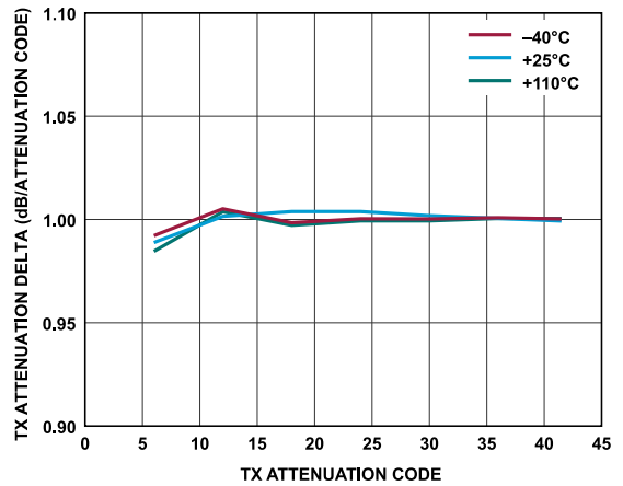
Figure 97. Transmitter Attenuation Delta vs. Transmitter Attenuation Code, Baseband Frequency = 18 MHz, Backoff = 0.2 dBFS
