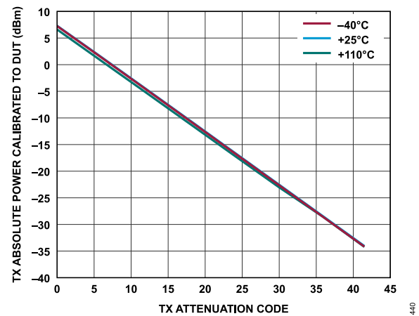
Figure 300. Transmitter Absolute Power Calibrated to DUT vs. Transmitter Attenuation Code, Baseband Frequency = 2.1 kHz, Backoff = 0.2 dBFS
