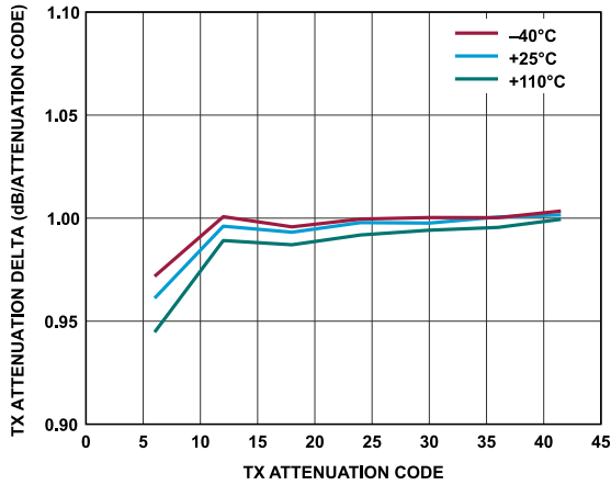
Figure 348. Transmitter Attenuation Delta vs. Transmitter Attenuation Code, Baseband Frequency = 2.1 kHz, Backoff = 0.2 dBFS
