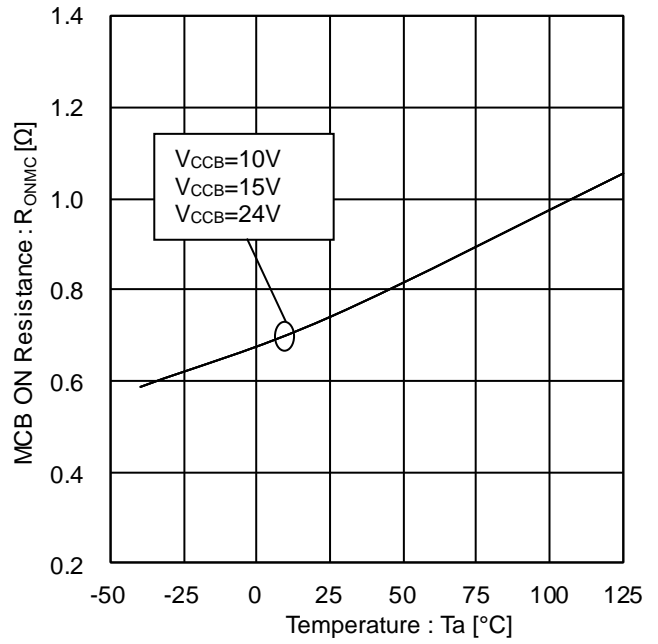
Figure 31. MCB ON Resistance vs Temperature
