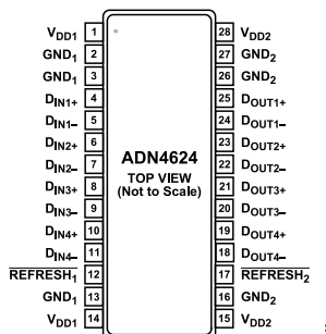
Figure 7. ADN4624 SOIC_W_FP Pin Configuration
