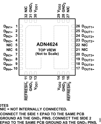
Figure 8. ADN4624 LFCSP Pin Configuration
