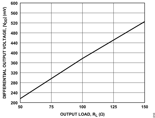
Figure 21. Differential Output Voltage, |V_{OD}| vs. Output Load, R_L (DC Input)
