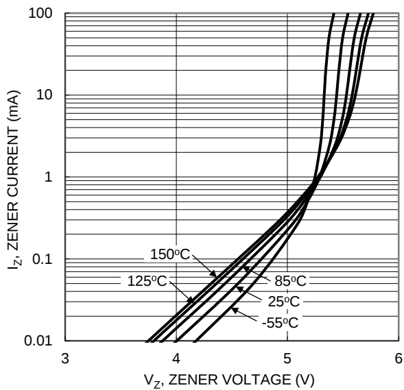
Fig. 3 Typical Reverse Characteristics DDZX5V6AQ
