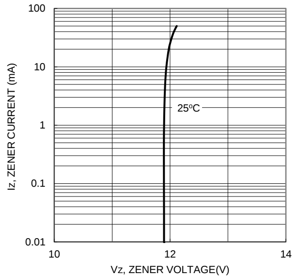
Fig. 4 Typical Reverse Characteristics DDZX12CQ
