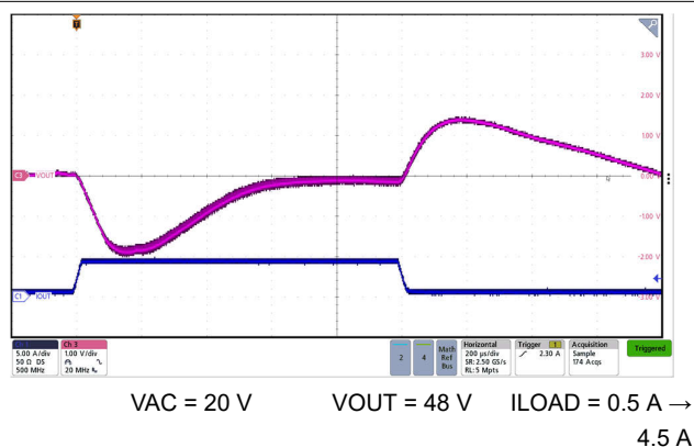
Figure 7-19. Forward Mode 48-V Transient Reponse with 20 Vin
