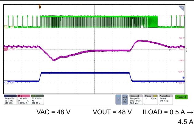
Figure 7-20. Forward Mode 48-V Transient Reponse with 48 Vin
