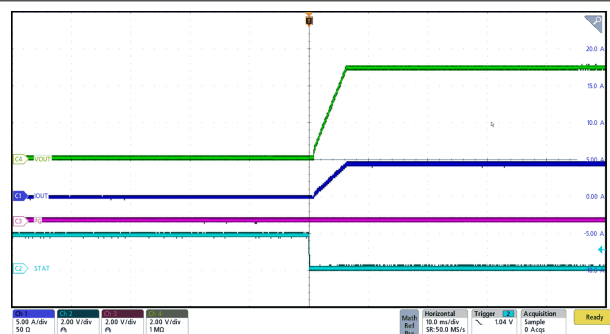
Figure 7-3. VAC Plug-In Power Up with 5-A Load
