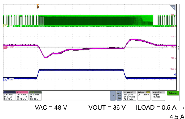
Figure 7-18. Forward Mode 36-V Transient Reponse with 48 Vin
