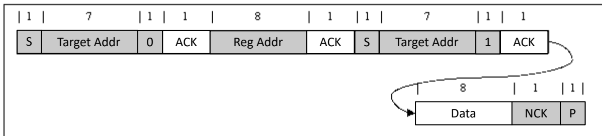
Figure 6-12. Single Read
