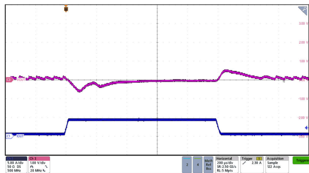
Figure 7-11. Forward Mode 5-V Transient Response with 20 Vin
