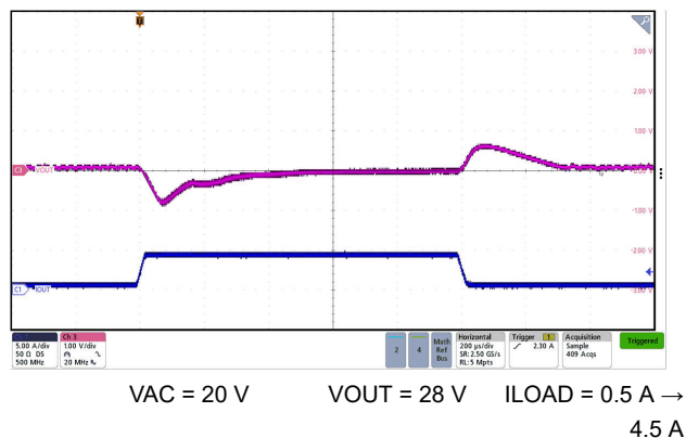
Figure 7-15. Forward Mode 28-V Transient Reponse with 20 Vin
