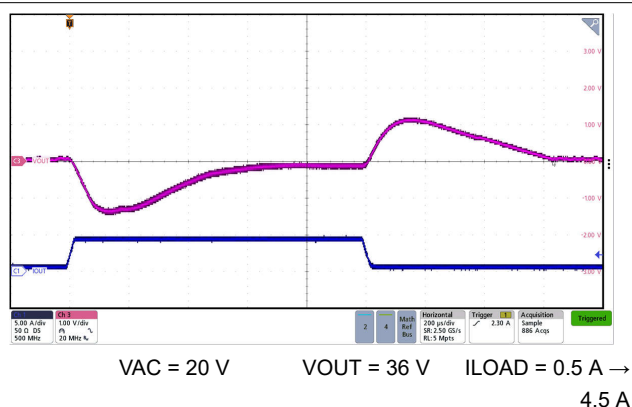
Figure 7-17. Forward Mode 36-V Transient Reponse with 20 Vin
