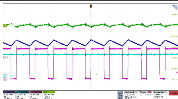
Figure 7-6. Power Down via I 2 C with 5-A Load
