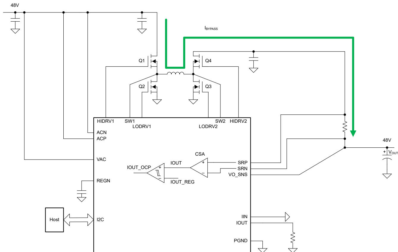
Figure 6-3. BQ25758 Bypass Mode Protection
