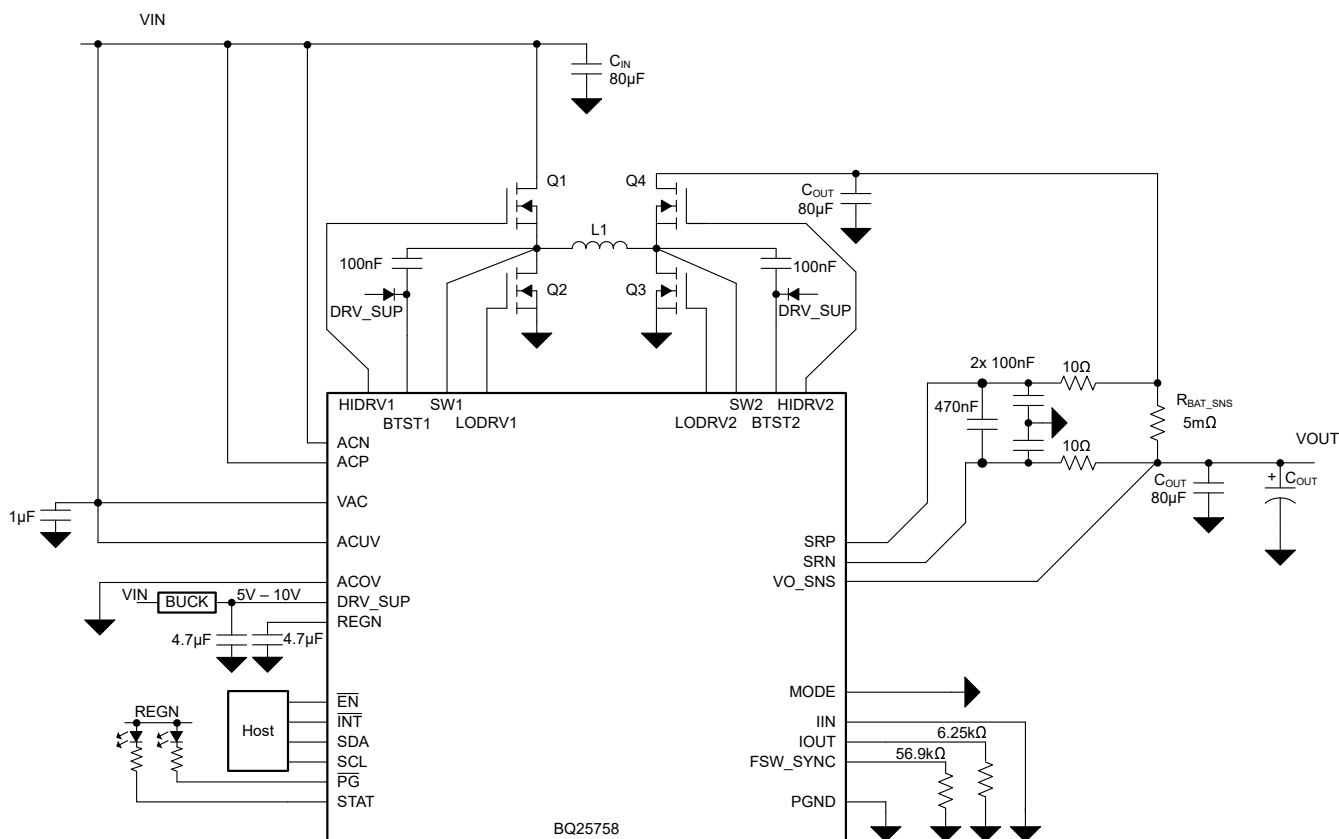
Figure 7-1. BQ25758: 19.5-V or 48-Vin, Buck-Boost with Configurable Output Voltage for USB-PD EPR, and 5-A Output Current
