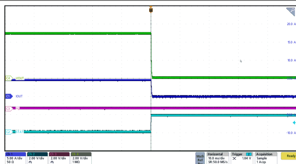
Figure 7-4. VAC Unplug Power Down with 5-A Load
