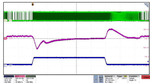
Figure 7-12. Forward Mode 5-V Transient Response with 48 Vin
