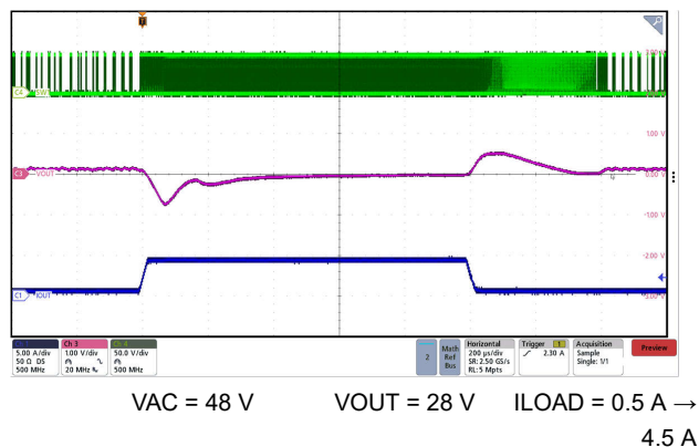
Figure 7-16. Forward Mode 28-V Transient Reponse with 48 Vin
