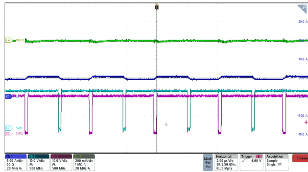
Figure 7-9. Buck-Boost Switching Waveform
