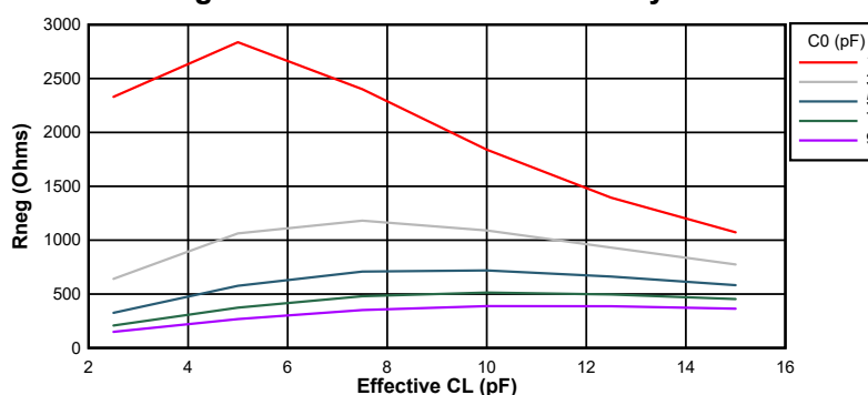
Figure 6-19. Negative Resistance Variation at 10 MHz
