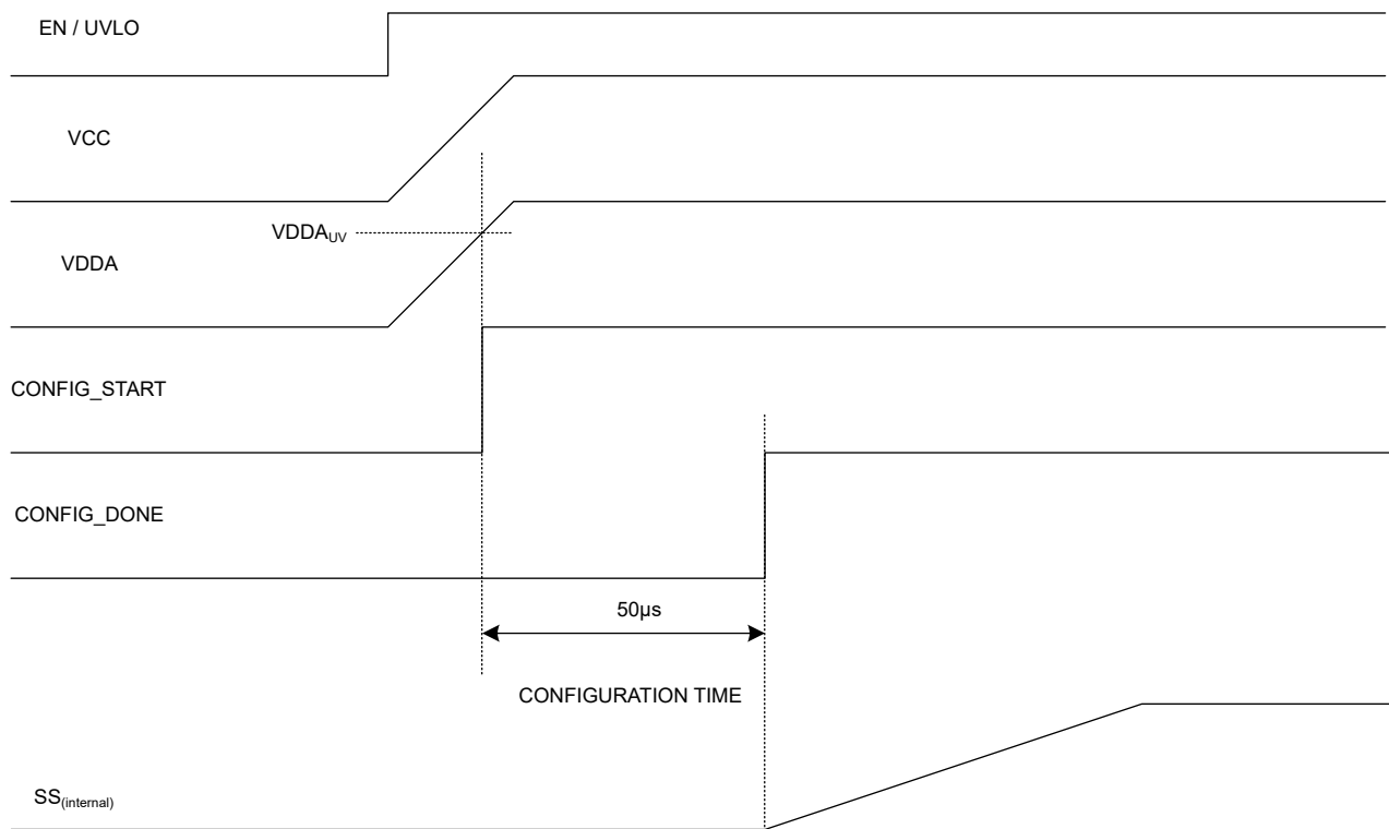
Figure 7-5. Configuration Timing
