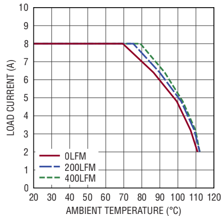
Derating Curve, V_{IN} = 12\text{V} , V_{OUT} = 1.5\text{V}
