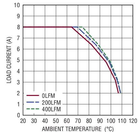
Derating Curve, V_{IN} = 12\text{V} , V_{OUT} = 2.5\text{V}
