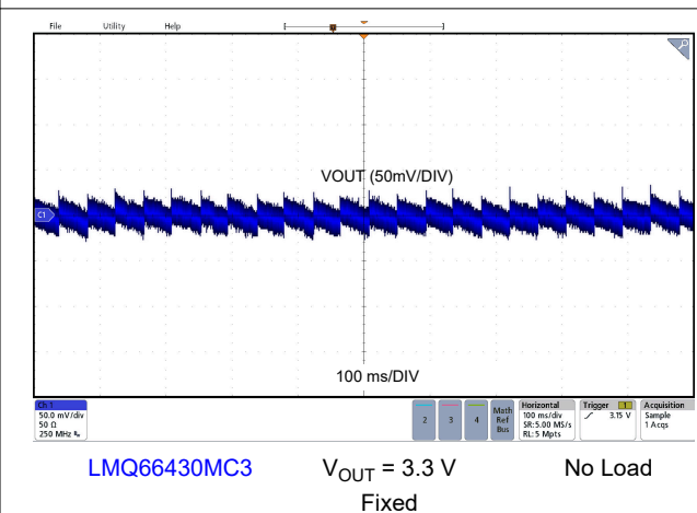
Figure 8-15. Output Voltage Ripple
