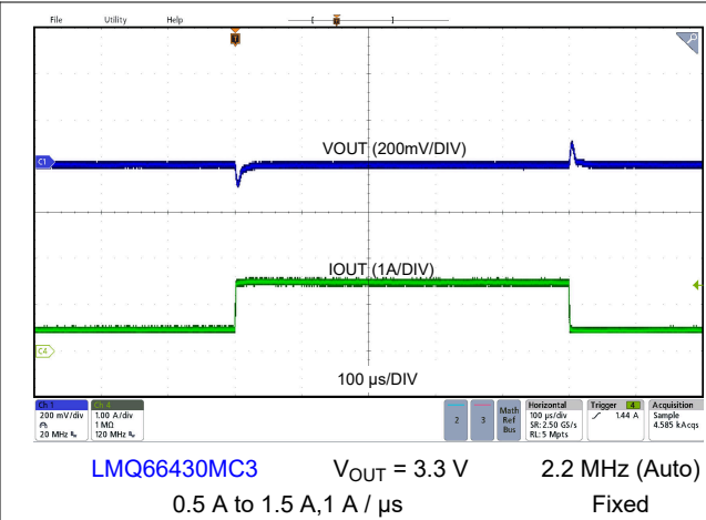
Figure 8-11. Load Transient
