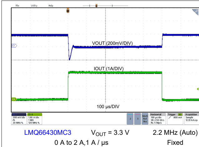
Figure 8-10. Load Transient
