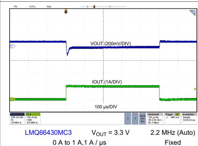
Figure 8-13. Load Transient
