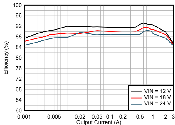
Efficiency: V_{OUT} = 3.3\text{V} (Fixed), 2.2MHz
