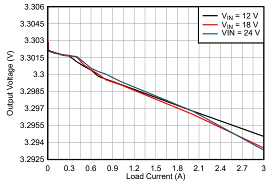
LMQ66430MC3 V_{OUT} = 3.3\text{ V} 2.2 MHz (Auto) Fixed
