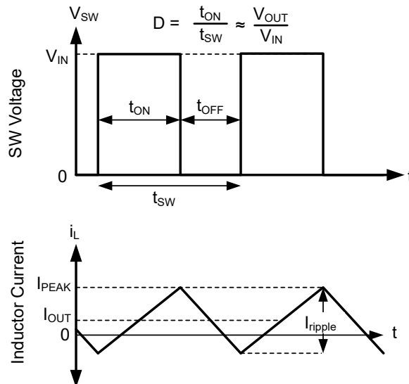
Figure 7-18. FPWM Mode Operation
