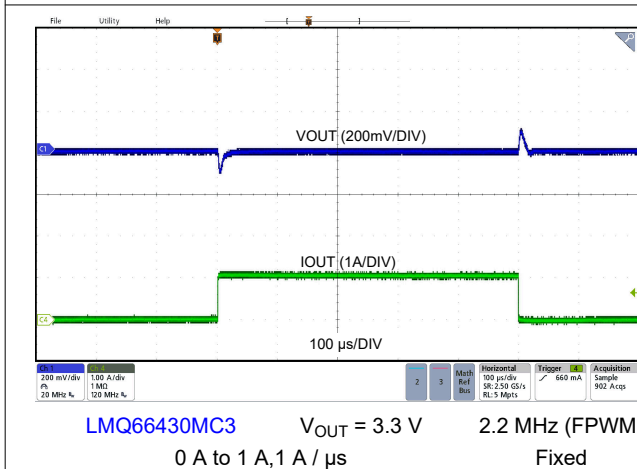
Figure 8-12. Load Transient
