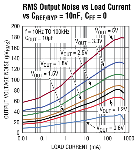
10Hz to 100kHz Output Noise C_{\text{REF/BYP}} = 10\text{nF} , C_{\text{FF}} = 0
