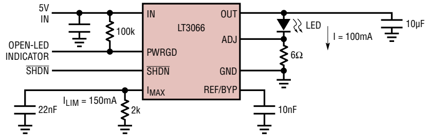
LED Driver/Current Source
