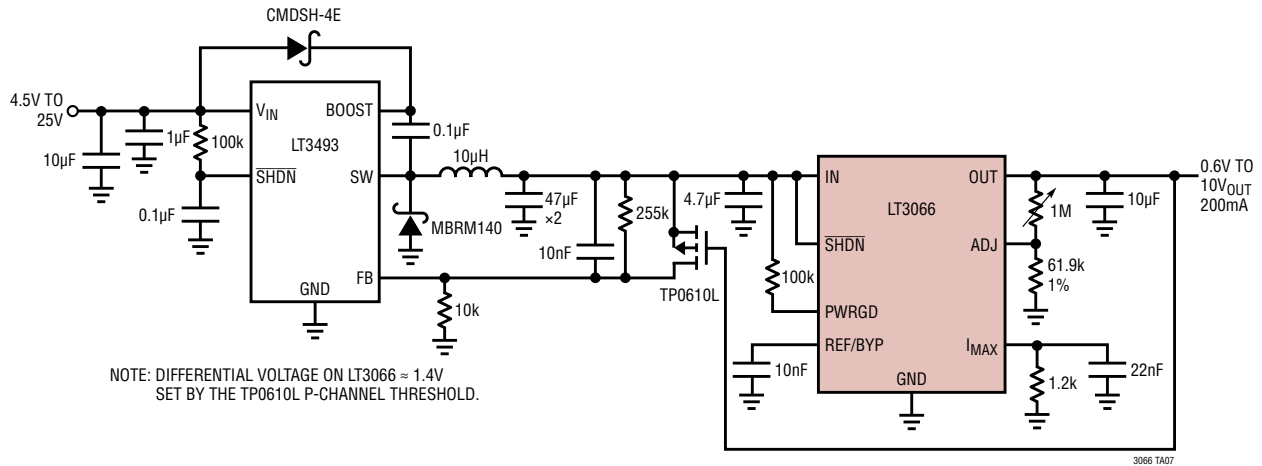
Adjustable High Efficiency Regulator
