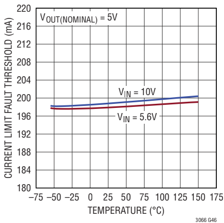
Precision Current Limit, R_{I\text{MAX}} = 1.5\text{k}
