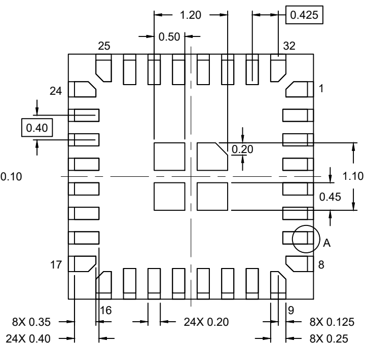
BOTTOM VIEW
