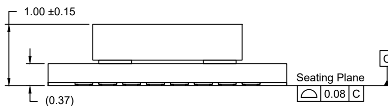
SIDE VIEW
