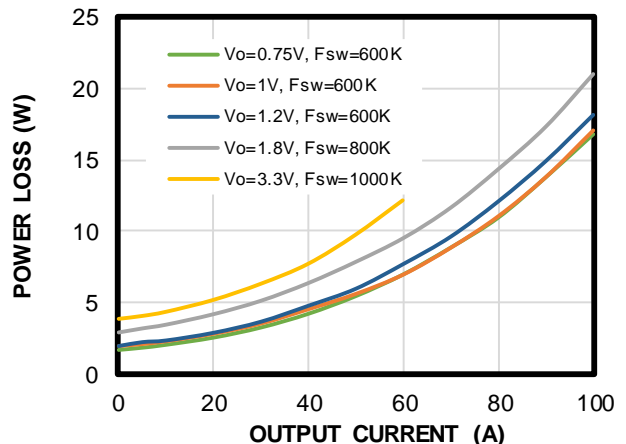
Power Loss vs. Output Current
