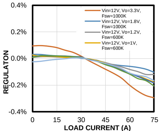
Load Regulation vs. Output Current
