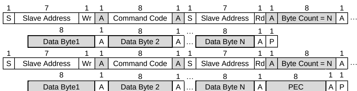
Figure 7: PMBus Message Format
