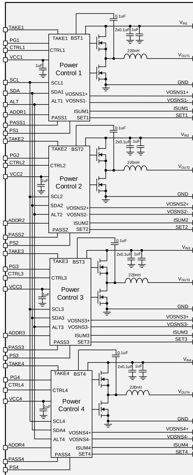
Figure 3: Functional Block Diagram
