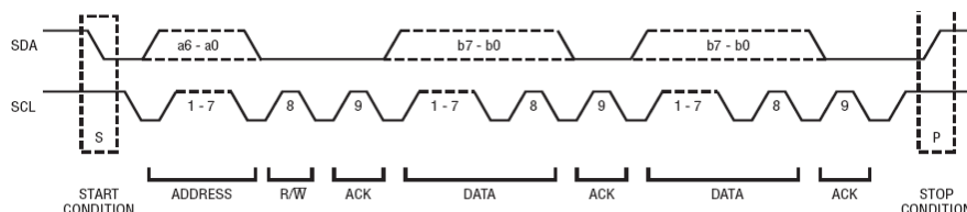
Figure 6: Data Transfer through the PMBus
