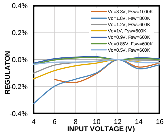
Line Regulation vs. Input Voltage
