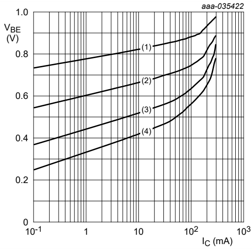
V_{CE} = 10\text{ V} (1) T_{amb} = -55\text{ }^\circ\text{C} (2) T_{amb} = 25\text{ }^\circ\text{C} (3) T_{amb} = 100\text{ }^\circ\text{C} (4) T_{amb} = 150\text{ }^\circ\text{C}
