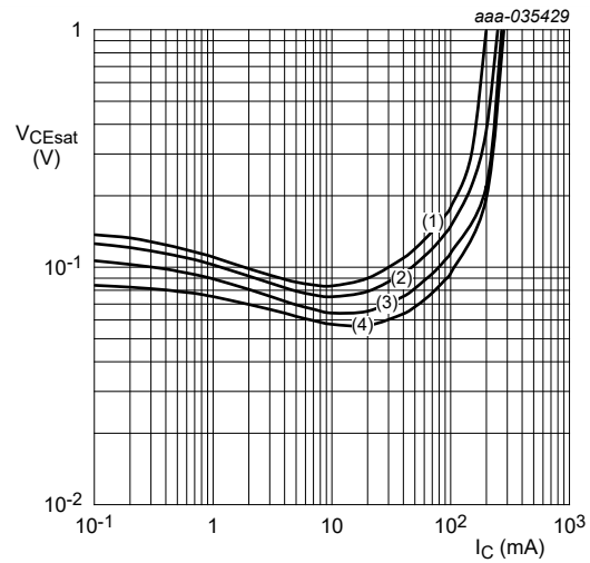
I_C/I_B = 10 (1) T_{amb} = 150\text{ }^\circ\text{C} (2) T_{amb} = 100\text{ }^\circ\text{C} (3) T_{amb} = 25\text{ }^\circ\text{C} (4) T_{amb} = -55\text{ }^\circ\text{C}
