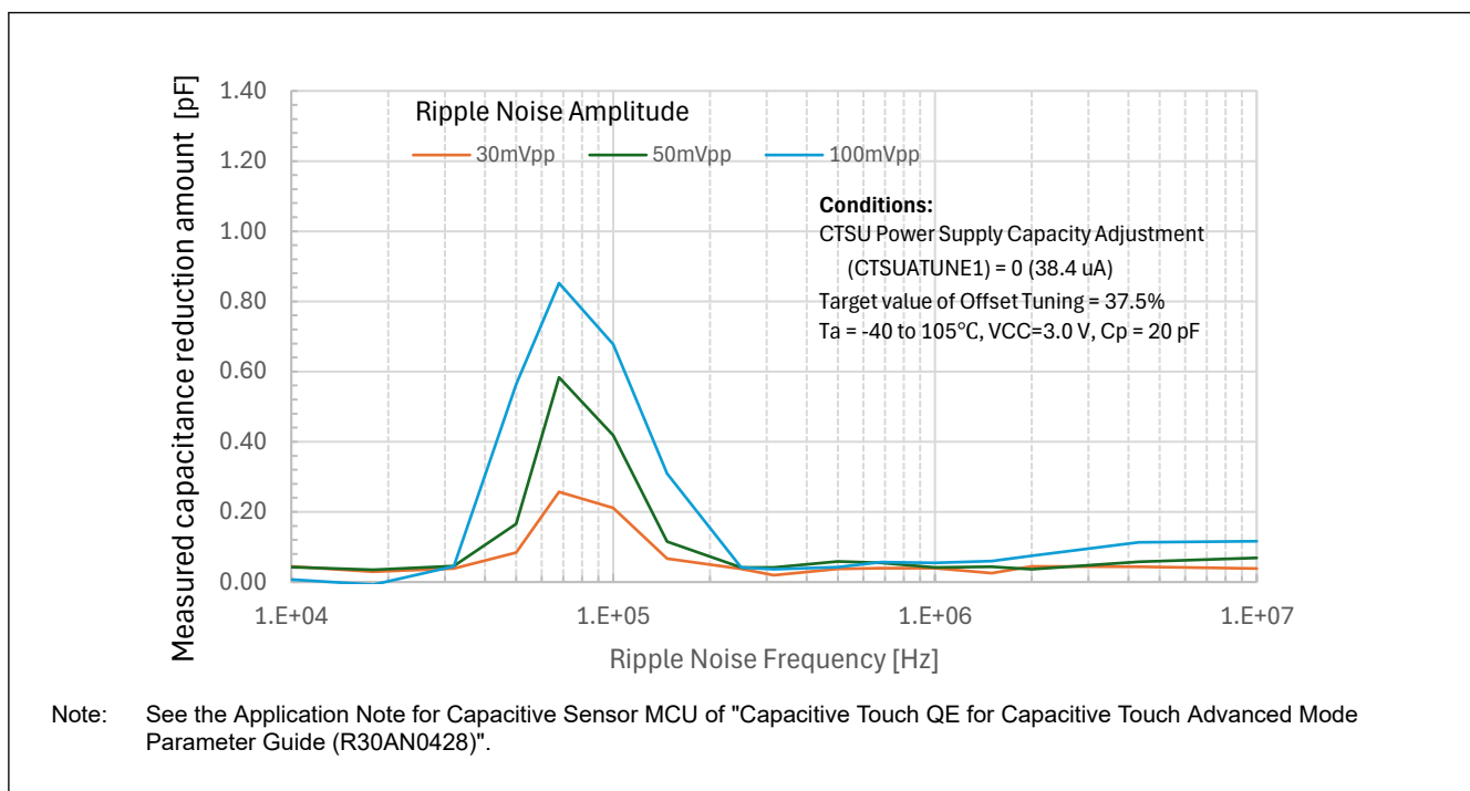
Figure 2.94 Measured capacitance reduction amount
