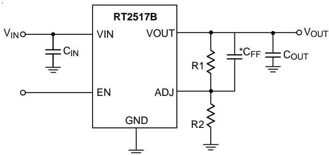
Figure 2. Application Circuit with C_{FF}
