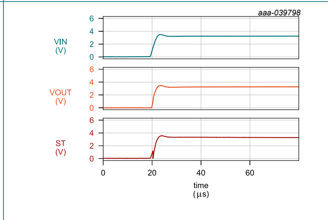
V_{IN} = 3.3\text{ V}; V_{EN} = 0\text{ V}; C_L = 100\text{ nF}; R_L = 1\text{ k}\Omega
