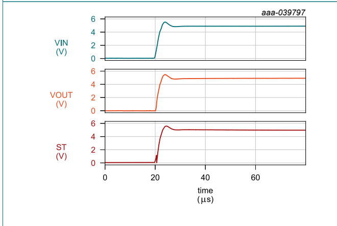
V_{IN} = 5\text{ V}; V_{EN} = 0\text{ V}; C_L = 100\text{ nF}; R_L = 1\text{ k}\Omega
