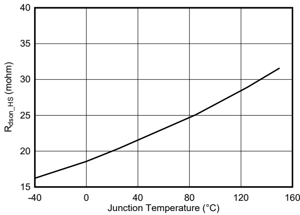
Figure 5-3. High-Side R_{DS(on)} vs Temperature
