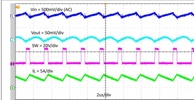
Figure 7-8. Steady State Waveforms, I_{OUT} = 4A
