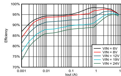
TPS56837 Efficiency, Vout = 5V, Fsw = 500kHz
