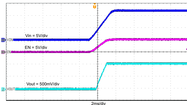
Figure 8-17. Start-Up with V_{IN} Rising, I_{OUT} = 3 A
