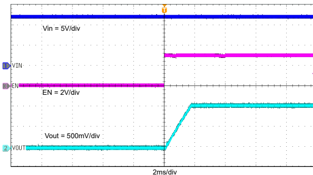
Figure 8-15. Start-Up Through EN, I_{OUT} = 3 A
