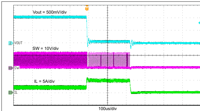
Figure 8-20. TPS563257 Normal Operation to Output Hard Short
