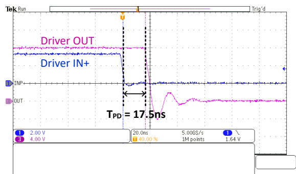
Figure 8-4. UCC27614 Falling (Turn-Off) Propagation Delay
