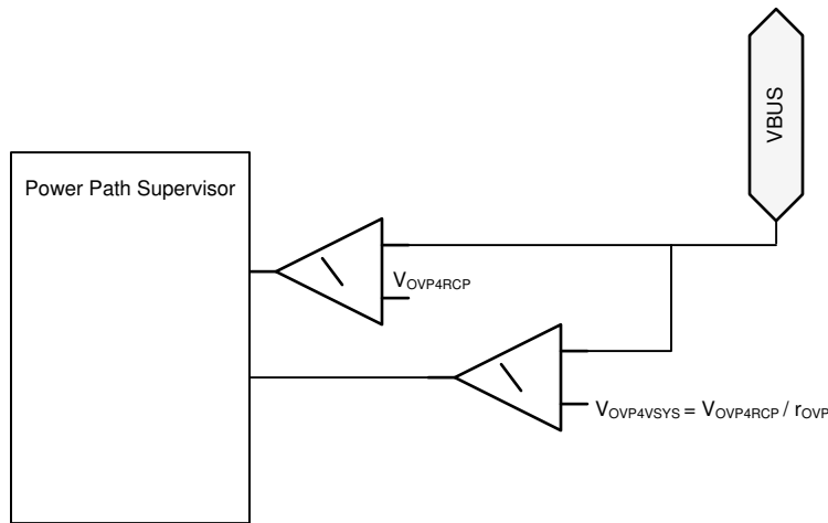
Figure 8-18. Diagram for OVP Comparators
