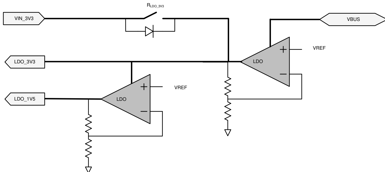
Figure 8-11. Power Supplies
