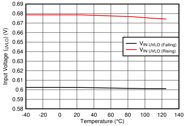
Figure 6-31. V UVLO(IN) Rising and Falling Threshold vs Temperature
