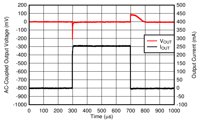
Figure 6-20. I_{OUT} Transient
