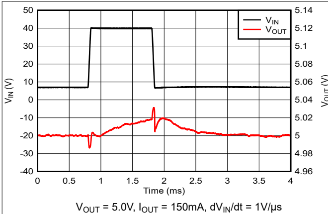
Figure 5-25. V_{IN} Line Transient (7V to 40V)
