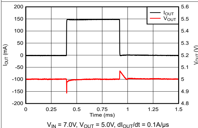
Figure 5-29. Load Transient (1mA to 150mA)
