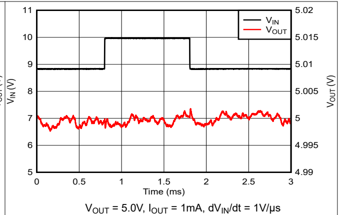
Figure 5-26. V_{IN} Line Transient (8.8V to 10V)
