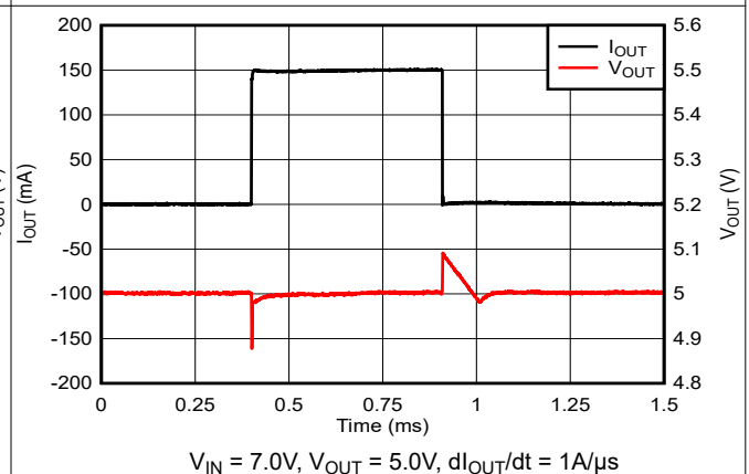
Figure 5-30. Load Transient (1mA to 150mA)
