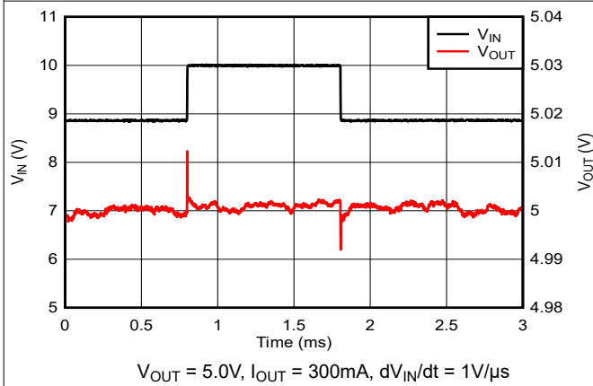
Figure 5-27. V_{IN} Line Transient (8.8V to 10V)
