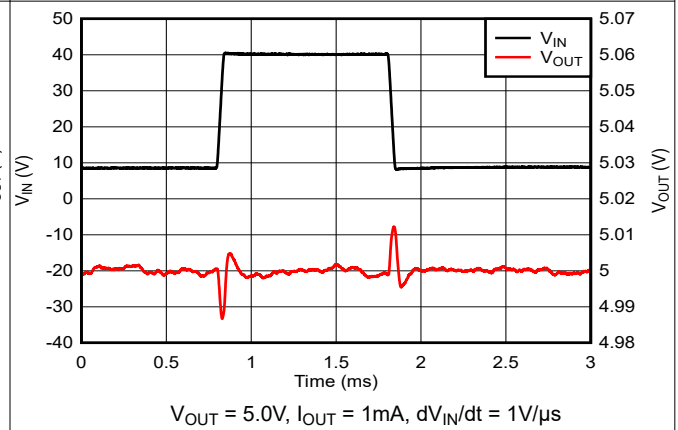
Figure 5-28. V_{IN} Line Transient (8.8V to 40V)
