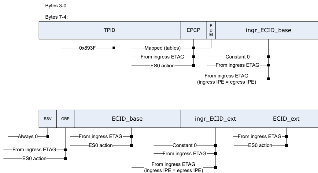
Figure 4-94. E-TAG Construction
