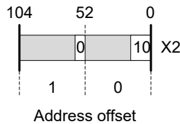
Figure 4-16. VCAP IP6PFX Entry Type-Group Fields
