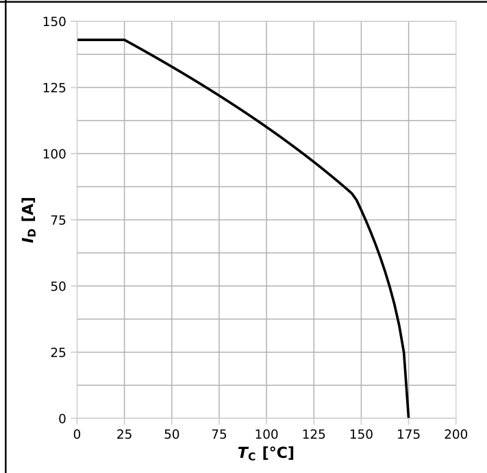
Diagram 2: Drain current
